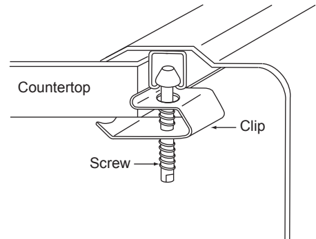
“U” Channel Type Installation Profile
