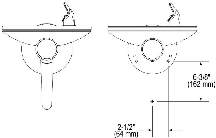
FRONT VIEWS
