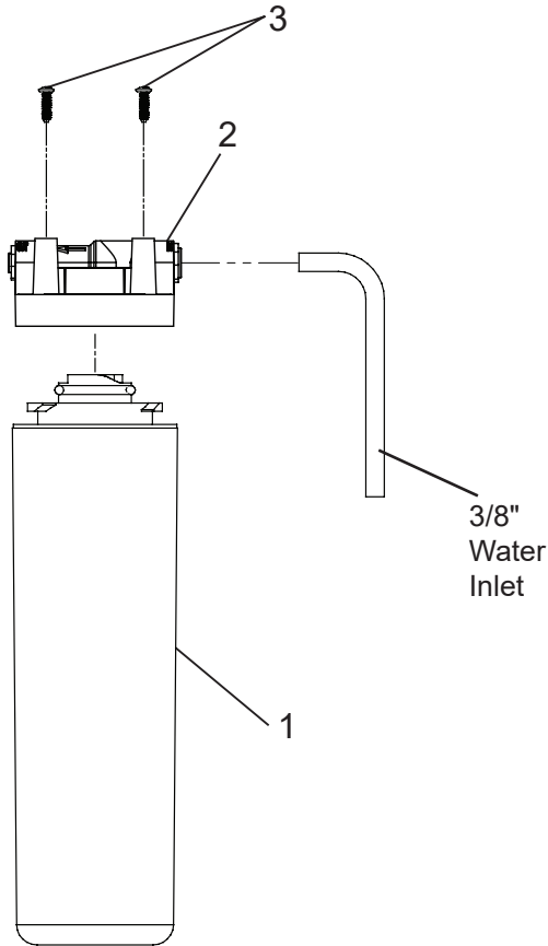
WATER FILTER EXPLODED VIEW FIG. 3
