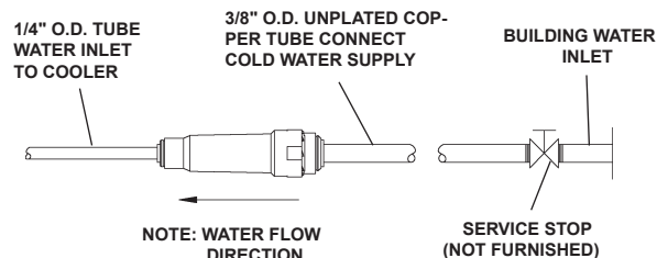
Figure 11 – Water Supply Connections
