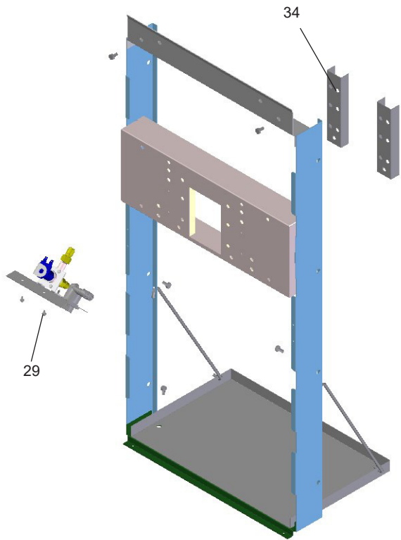
Figure 7 - Solenoid Assembly
