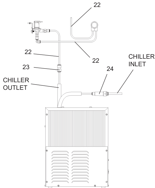
Figure 3 - ENO Tube Routing
