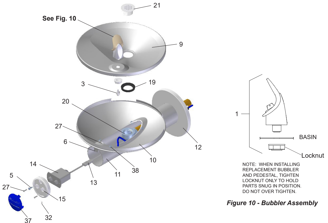
Figure 9 - Exploded View
