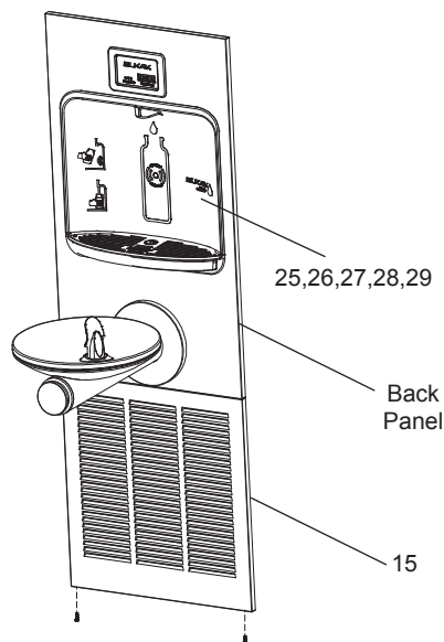
Figure 4 - Lower Panel Installation
