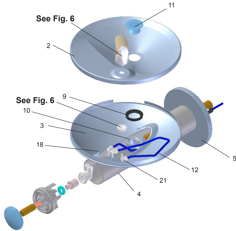
Figure 5 - Fountain Body Assembly
