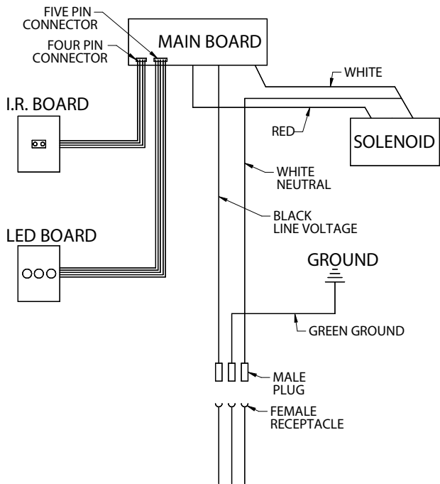
Electrical Diagram
