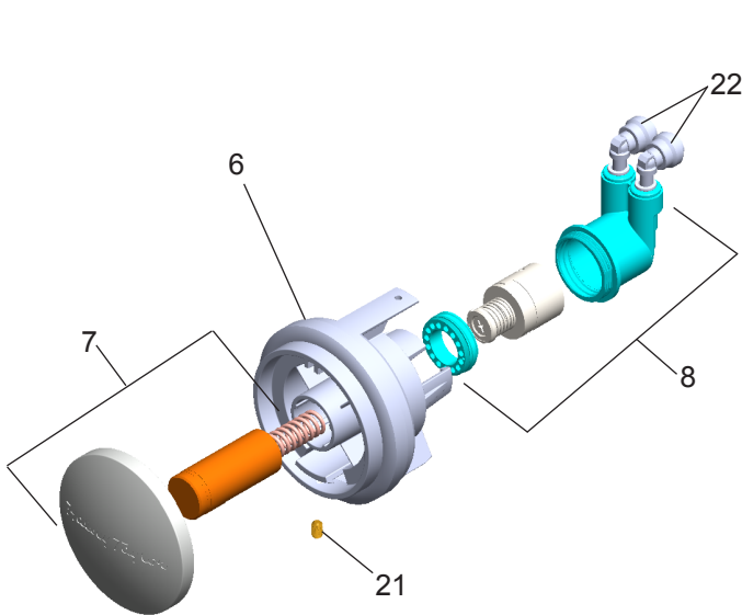
Figure 8 - Push Button Assembly
