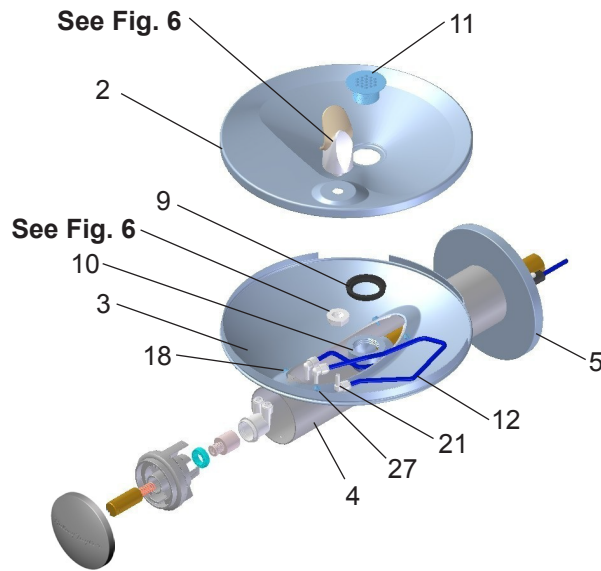
Figure 8 - Fountain Body Assembly
