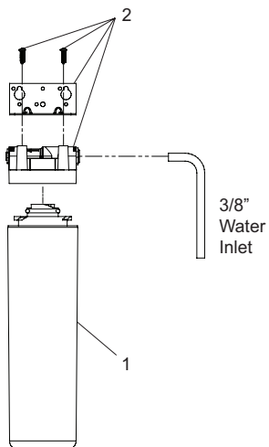
Filter Head Assembly used after 01/01/2021
