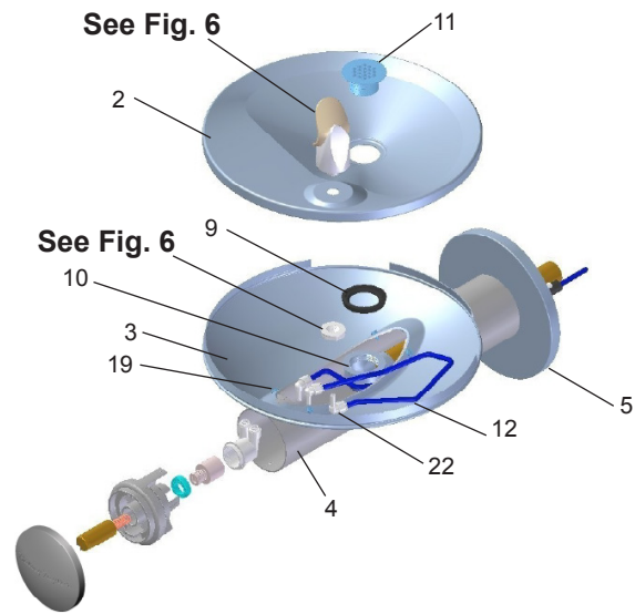
Figure 7 - Fountain Body Assembly
