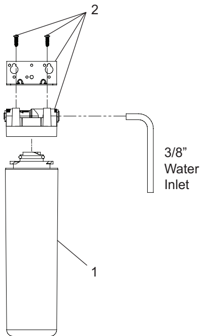
Filter Head Assembly used after 01/01/2021
