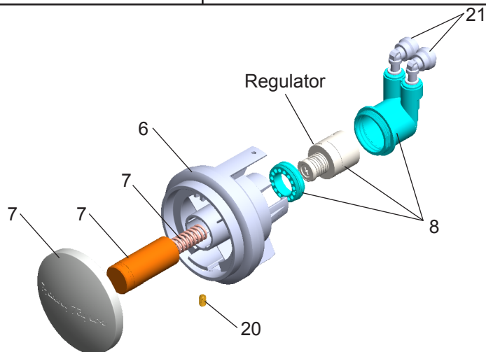
Figure 9 - Push Button Assembly
