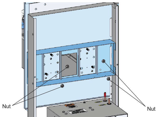
Figure 7 – Fountain Installation
