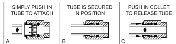
Figure 11 – Filter Quick Connect Fittings
