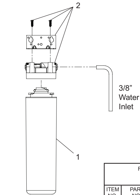
Filter Head Assembly used after 01/01/2021
