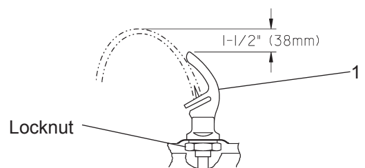
Figure 6 - Bubbler Detail
