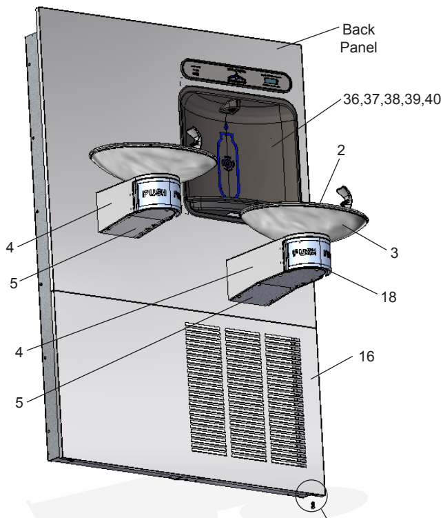
Figure 5 Lower Panel Installation
