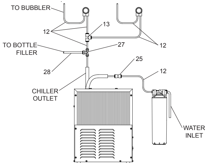
Figure 3 - HTHBWF-OVLSEWSI-I Tube Routing
