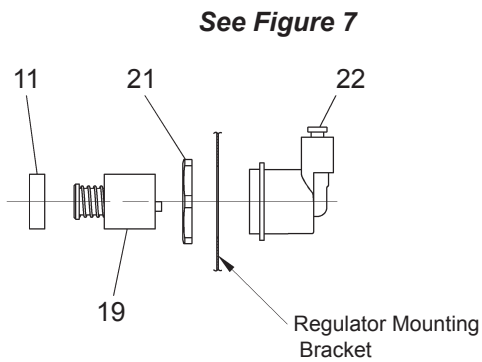
Figure 9 Regulator Assembly
