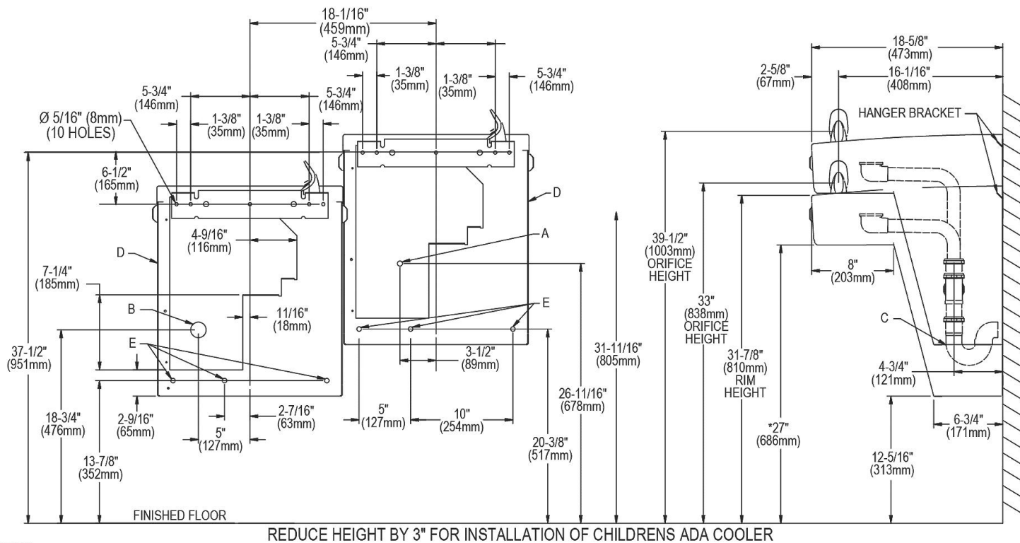
REDUCE HEIGHT BY 3" FOR INSTALLATION OF CHILDRENS ADA COOLER
